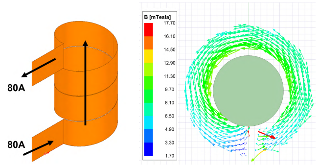
Fig. 4: Net z-directed current for an example design carrying 80A (left). Phi-directed field component in the outer shell due to the z-directed current, estimated to be 12mT, considerably larger than the z-directed field component, measuring 3.5mT (right)
