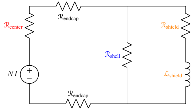
Fig. 2: Magnetic circuit model for the self-shielded inductor. The alternating core pieces and gaps in center post and outer shell are modeled as lumped reluctances. The lossy nature of the shield is modeled as a transference element \mathcal{L}_{\text{shield}} [18], [19].
