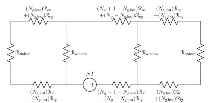
Fig. 7: Refined magnetic circuit model for z-directed fields accounting for the additional inductance due to lost gaps.
