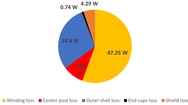
Fig. 9: Loss distribution in the optimized inductor, the total loss is 85 W. This analysis doesn't include dielectric loss.
