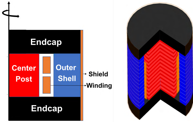
Fig. 1: Radial cross-section of the proposed inductor design, featuring the center post, outer shell, end caps, copper shield and a single-layer winding (left). 3D model with a transparent shield and a pie cut out for better visibility (right). The outer shell has notches that are not visible in these views.
