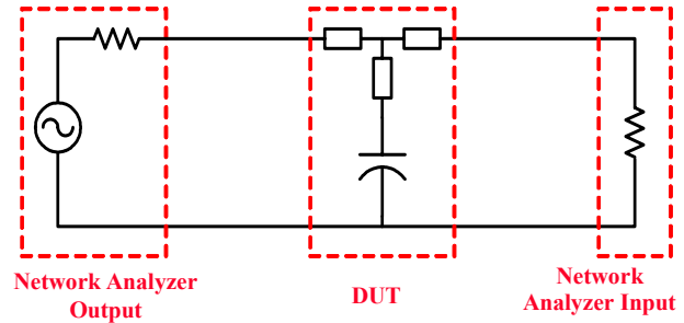
Fig. 7. An experimental setup for evaluating filters and components incorporating an Agilent 4395A network analyzer. The device under test (DUT) comprises a filter capacitor and a printed circuit board inductance cancellation transformer with their interconnects.
