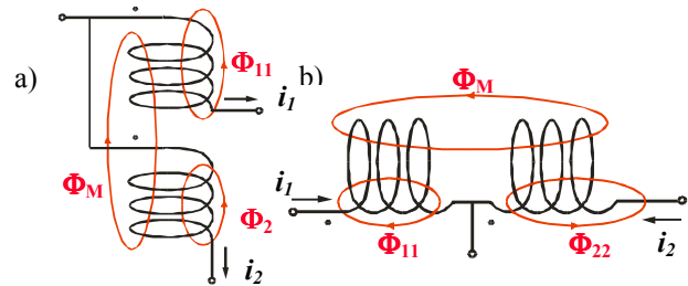
Fig. 1. (a) An end-tapped and (b) a center-tapped connection of coupled magnetic windings.
