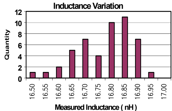
Fig. 4. A histogram of the parasitic inductances found for Beyschlag Centrallab 2222 338 24 224 X-type capacitors (0.22 \mu\text{F} , 275 Vac). The average value is 16.81 nH, with a standard deviation of 112 pH.
