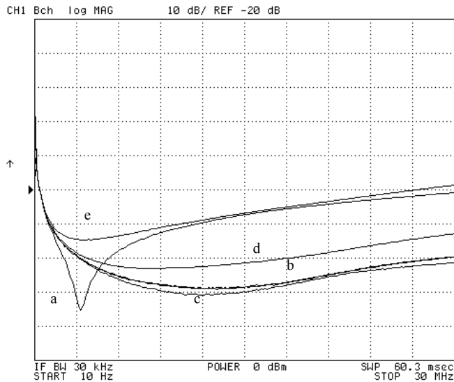
Fig. 13 The effects of magnetic material on the performance of inductance cancellation. Signal a shows the performance of a capacitor with no inductance cancellation windings, while signal b shows the performance with cancellation. When a ferrite core is placed adjacent to the capacitor and air-core windings there is not much change (c). The maximum amount of interference occurs when the core impinges directly on the windings. When the core is approximately 100 mils from the coils (d) the performance drops. When the core is placed directly over the windings, inductance cancellation is completely ineffective (e).
