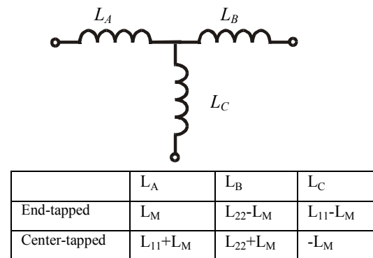
Fig. 2. An equivalent circuit model for the configurations of Fig. 1.
