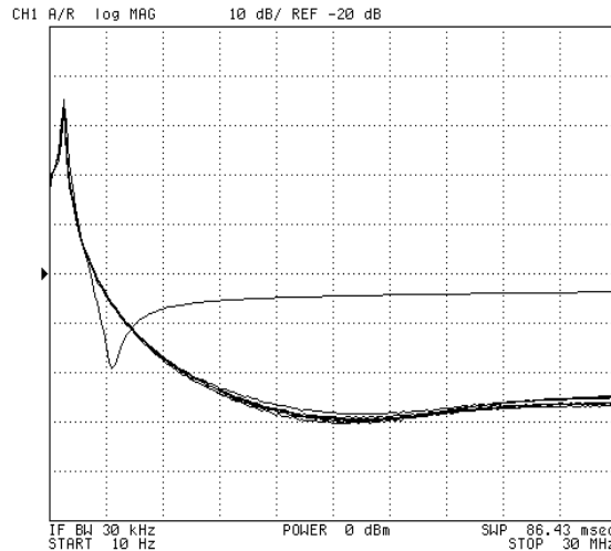
Fig. 10 Repeatability curves. The higher curve is a capacitor alone (no cancellation). The lower curves are results with six nominally identical circuits incorporating printed cancellation windings. Note that the curves are all within 3 dB of each other.
