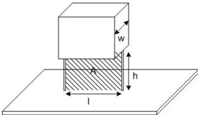
Fig. 6 The parasitic inductance created by lifting the capacitor off the board can be approximated using l , h , w , and \mu_0 .
