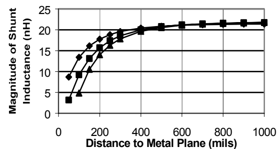
Fig. 12 The effect of a metal plane on the effective negative shunt inductance. The results are for the transformer designs used in Table 1. The highest curve shows the effect for a center-tapped transformer. The two coils for an end-tapped core are always different. One coil must have a low inductance, while the other is very high. The middle curve is shows the effect for the end-tapped core in which the metal plane is approaching the low-inductance coil. The lowest curve shows the effect when the plane approaches the high-inductance coil of the transformer.
