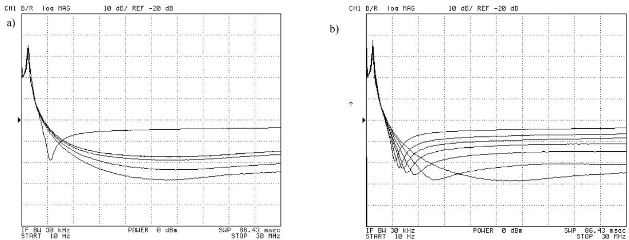
Fig. 9 The highest curve in both Fig. 9a and 9b represents the performance of a capacitor without any inductance cancellation in the test setup of Fig. 7. The curves in Fig. 9a are the results with center-tapped transformers having mutual inductances between 6 nH and 26 nH at intervals of 4 nH each. Figure 9b shows the results of having a mutual inductance that is too large; these curves are the results with transformers having mutual inductances between 26 nH and 32 nH with intervals of 2 nH.
