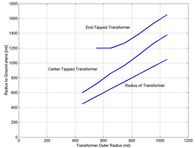
Fig. 11 The amount of spacing that is needed between the transformer and the groundplane to ensure that the shunt path inductance is within 1dB of its desired value. The lowest curve represents the outer edge of the transformer coil. The spacing needed for a center-tapped transformer is about 33% larger than the outer radius of the transformer. The radius needed for end-tapped designs is larger
