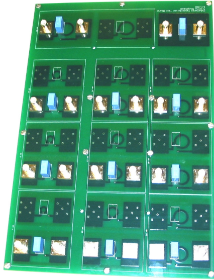
Fig. 8 A test comparison board. A capacitor without inductance cancellation is in the upper right corner. Every other layout has a transformer with a different shunt path inductance
