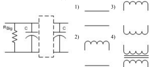
Fig. 14 The EMI filter under test. The box can be replaced by any of the four connections, as shown. The filter can also use capacitors with or without inductance cancellation.
