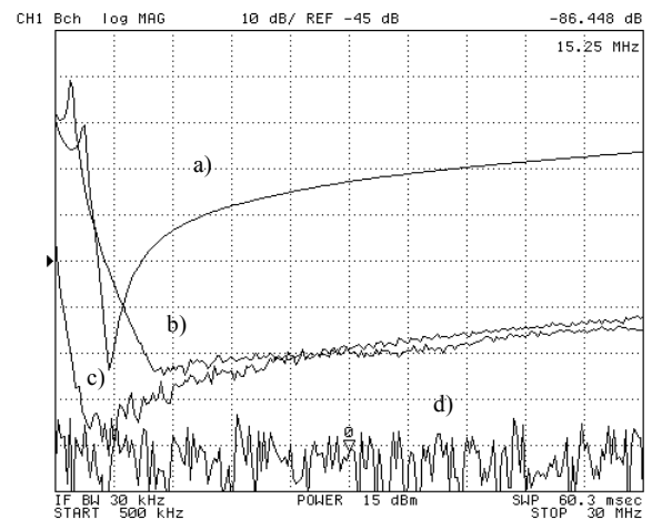
Fig. 16 The results of the EMI Filter test. Signal a is the performance of two normal capacitors. Signal b is the performance of two capacitors with inductance cancellation. Signal c is the performance of a normal capacitor with a single inductor in the series path. Signal d is the noise floor.
