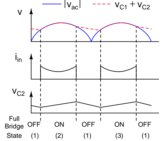
Fig. 2. The figure illustrates the three states and operation of the stacked ac-dc converter system. The waveform shows input current and voltage across capacitor C_2 waveform across the line cycles.
