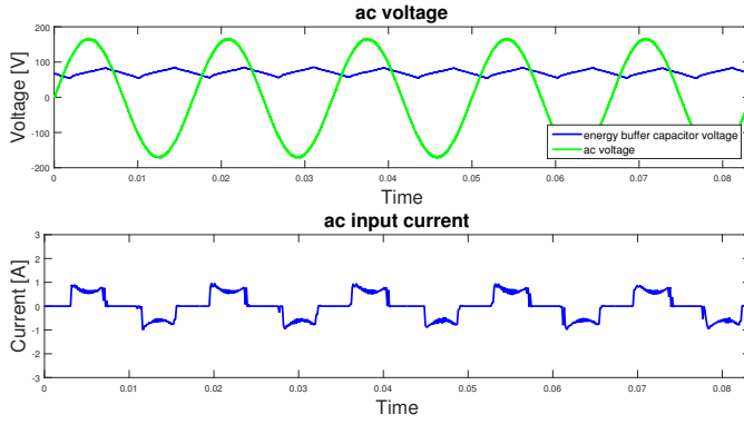
Fig. 10. The figure shows the measured waveforms when the converter operates at 120\text{ V}_{\text{ac}} and supplies 48\text{ W} at 12\text{ V}_{\text{dc}} system output. The waveform shows the ac line voltage, the voltage across the energy buffer capacitor, and the input ac line current waveform over the line cycle.
