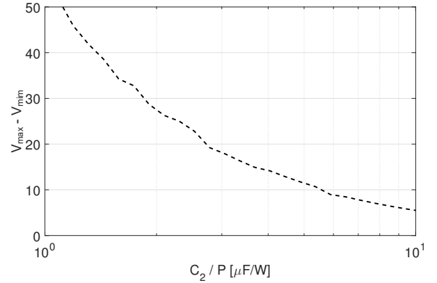
Fig. 4. This figure illustrates the relation between the voltage swing across the energy buffer capacitor and its capacitance (e.g., K_{c2p} = C_2/P_{out} ) when the K_{c1p} = C_1/P_{out} = 0.2 [\mu F/W] and the converter operates at 120 Vac input voltage and dc output power P_{out} . As shown in the graph, a smaller energy buffer capacitor increases the voltage fluctuation over the line cycle, such that the following regulating converters need to operate across wider voltage ranges.
