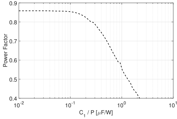
Fig. 3. The figure shows the achievable power factor of the voltage-regulated system with different C_1 values at the given power level (e.g., K_{c1p} = C_1/P_{out} ) when K_{c2p} = C_2/P_{out} = 2 [\mu F/W] . This figure illustrates the effect of small capacitance values (i.e., C_1 , the capacitor stacked with the main energy buffer capacitor C_2 ) on the achievable power factor. It can be seen that larger C_1 values degrade power factor for a given power level and C_2 capacitance value.
