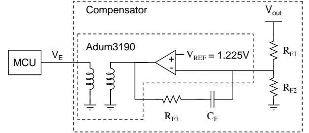
Fig. 7. The figure shows the PI compensator design with isolated error amplifier (Adum3190 from Analog devices which also provides a 1.225 V reference voltage). The voltage divider values are selected such that R_{F1}/(R_{F1}+R_{F2}) V_{out} = 1.225 V and the transfer function of this compensator is as shown in Fig. 8.
