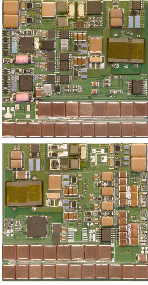
Fig. 9. The ac-dc isolated converter is implemented on a 2.1 in(x) \times 1.95 in(y) \times 0.22 in(z) converter box volume using the ceramic energy buffer capacitors. This figure shows the top and bottom side of the PCB illustrating several components: (1) energy buffer capacitor, (2) GaN transistors, (3) Silicon Schottky diode, (4) regulating converter inductor, (5) Full-bridge and EMI filter, (6) planar transformer, and (7) capacitively-aided isolated converter.
