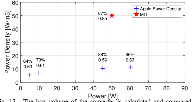
Fig. 12. The box volume of the converter is calculated and compared to the conventional isolated ac-dc converters for applications such as battery chargers from Apple. The prototype converter can achieve five times higher power density with 30–100 times higher switching frequency operation.
