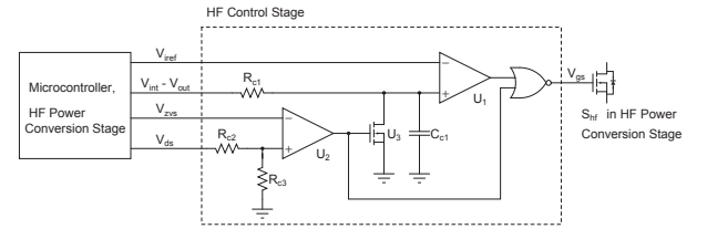
Fig. 8. Schematic of the HF regulation control circuit. This control circuit is designed to regulate the average inductor current by changing the switch on-time, and to operate the HF stage at zero-voltage or near zero-voltage switching conditions. Comparator U_1 triggers the switch turn-off event, and comparator U_2 triggers the switch turn-on event.
