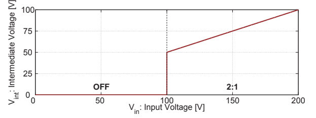
Fig. 3. The voltage transformation characteristic of the switched capacitor (first) stage in an ac-dc converter. The SC circuit is operated with 2:1 conversion ratio only when the input voltage goes above 100 V and is turned off for lower input voltages.
