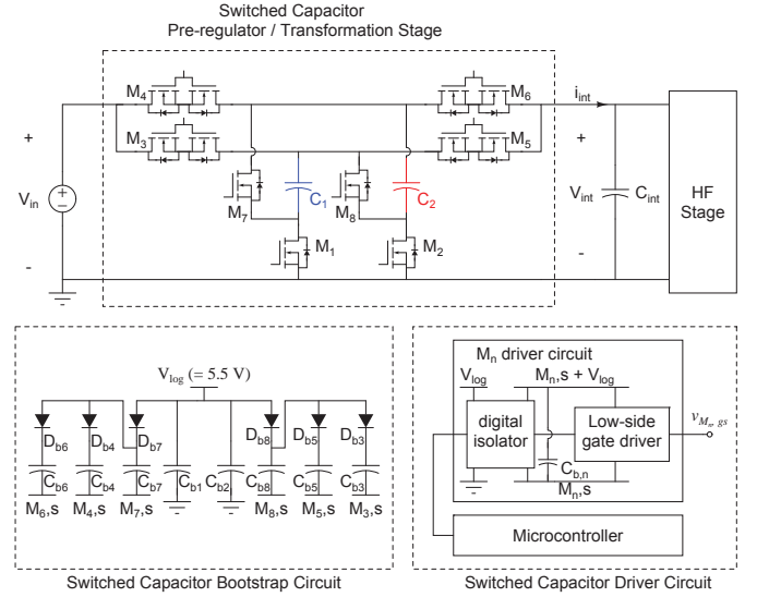
Fig. 5. The switched capacitor circuit comprises transistors, energy transfer capacitors, and bootstrap diodes and capacitors. The switches M_3 - M_6 are realized with back-to-back connections of two transistors to block bidirectional voltage. For the control circuitry, the logic power supply V_{log} (= 5.5V) is applied to a set of bootstrap diodes and capacitors to generate appropriate floating supplies for driving the transistors. It should be noted that this bootstrap configuration applies for all conversion modes.
