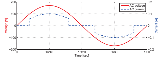
Fig. 10. Waveform of the sinusoidal ac voltage and a “clipped sine wave” ac current. The clipped-sinewave current pattern operating over a 108 degree range for each 180 degree half-cycle yields a power factor of 0.95 (this corresponds to a 100 V “cut in” voltage for a 170 V peak sinusoidal voltage). Operating over a 120 degree range per half-cycle yields a power factor of 0.97.
