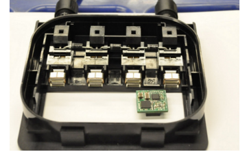
(b) Photograph showing discrete implementation of the power converter together with a solar panel junction box.
