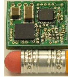
(a) Photograph of the sub-module MPPT converter with pencil shown for scale. The power inductor is on the bottom side of the PCB.
