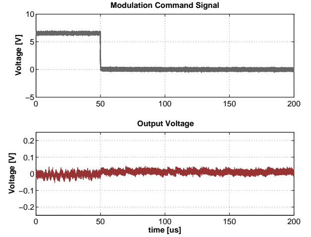
(a) 0.5 W to 3.5 W load step
